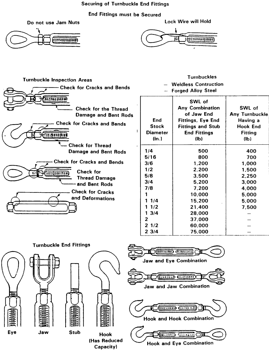
Figure 10-11. Turnbuckle Types, Inspection Areas, and Safe Working Load.
