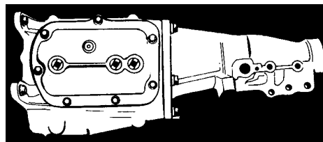
456 SAGINAW TORQUE TUBE TAILSHAFT, G.M., 81-82 CAMARO/FIREBIRD 7 bolt side cover
